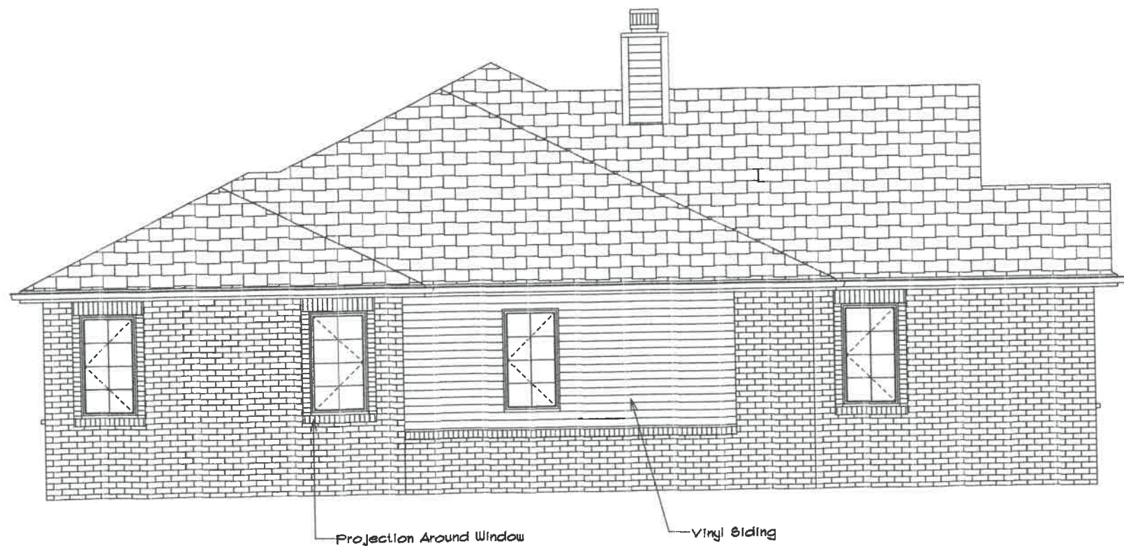
LEFT ELEVATION
